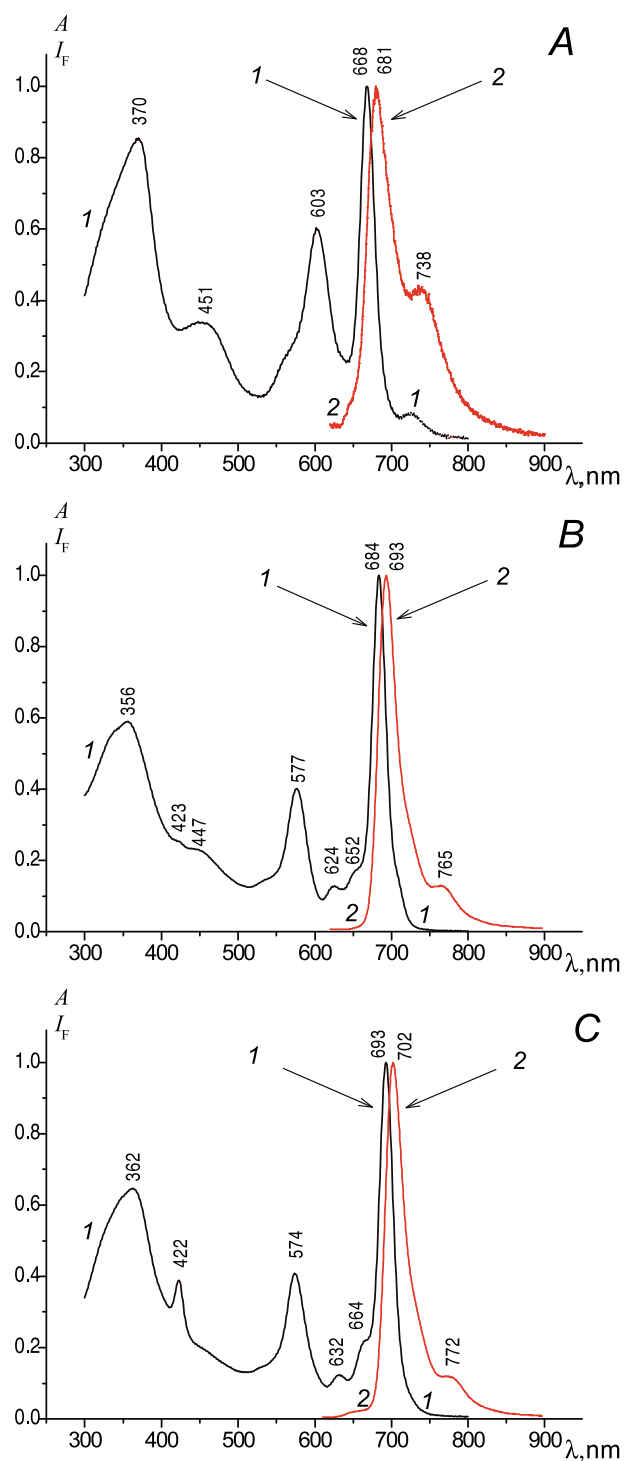
Figure 1. Absorption (1) and fluorescence (2) spectra of H_2PAPh_8 (A, \lambda_{exc}=602 nm), H_2\{SN_2\}PAPh_6 (B, \lambda_{exc}=577 nm) and H_2\{SeN_2\}PAPh_6 (C, \lambda_{exc}=574 nm) in toluene at 293 K.
